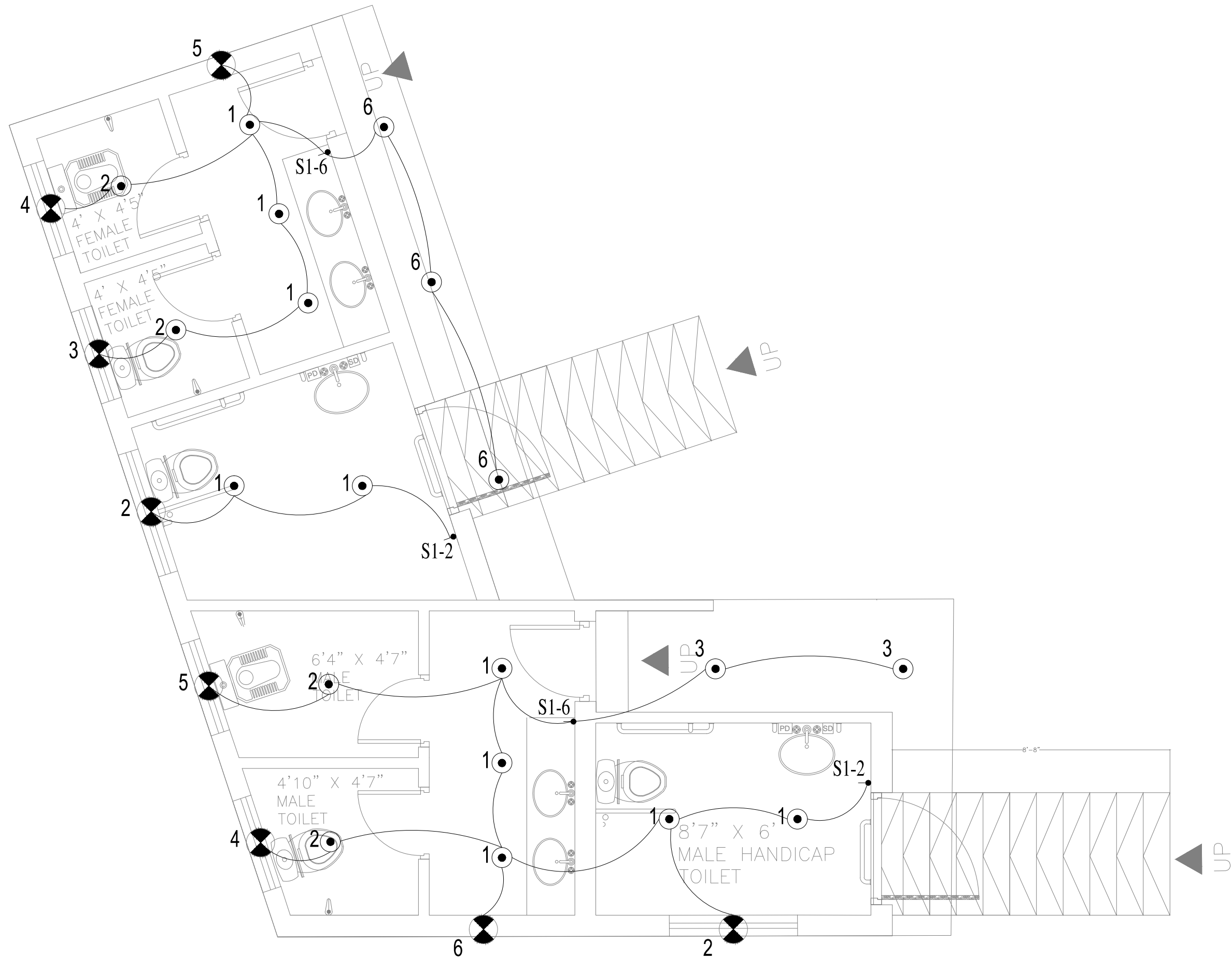
TOILET BLOCK WORKING PLAN
