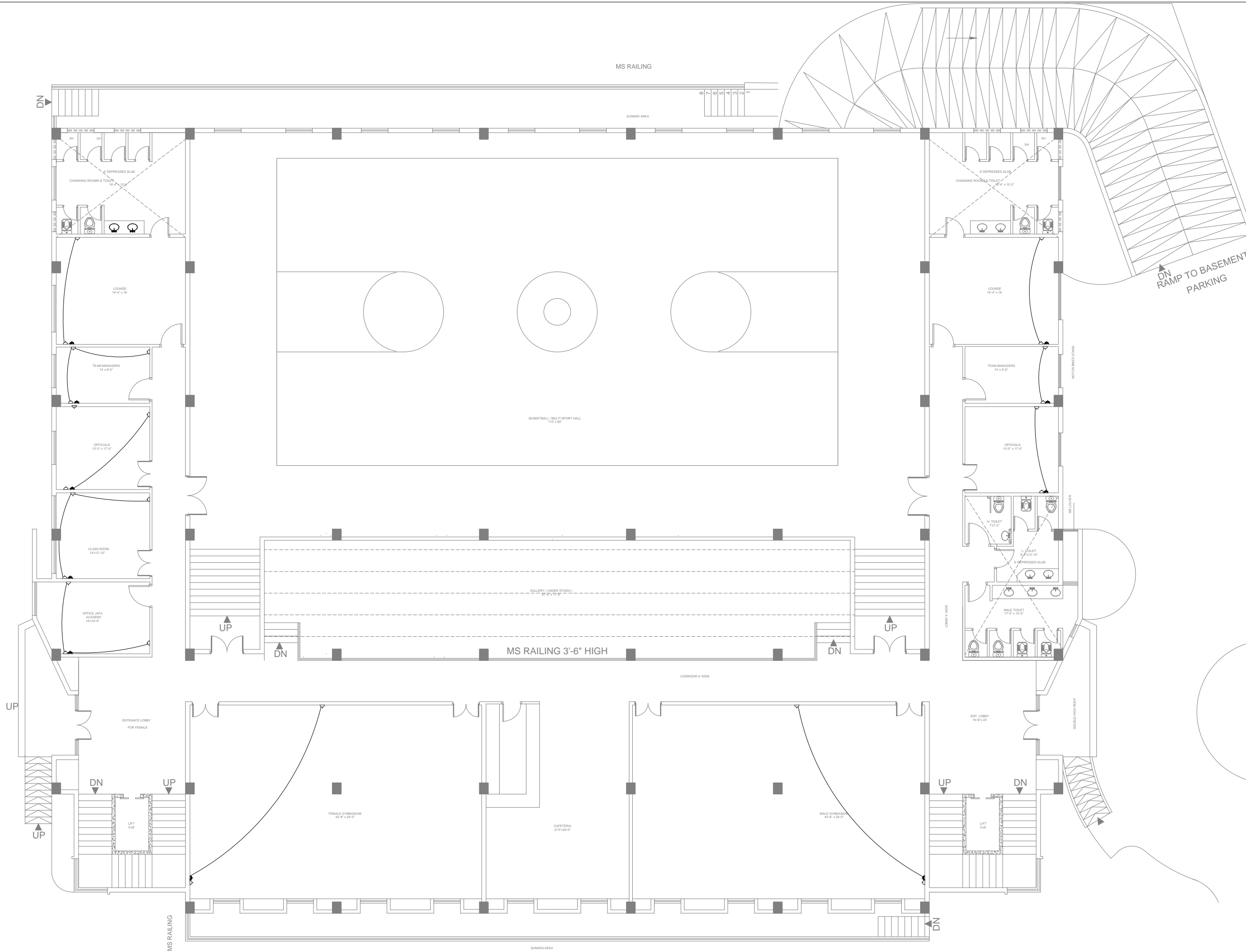
GROUND FLOOR PLAN COVERED AREA 10,975 SFT
