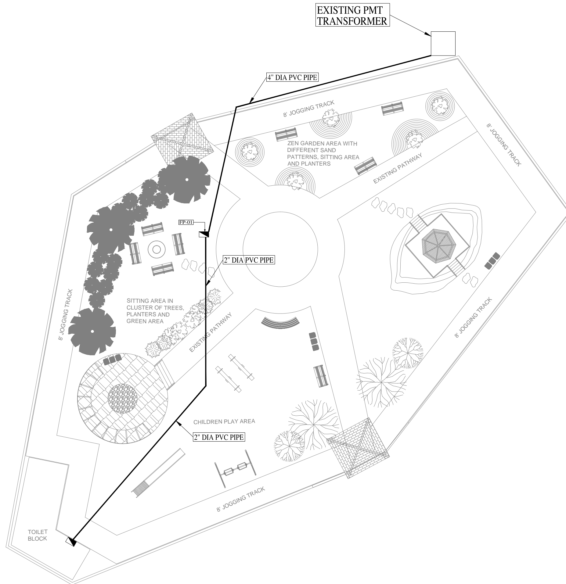
ALLAH RAKHA PARK – WORKING PLAN
